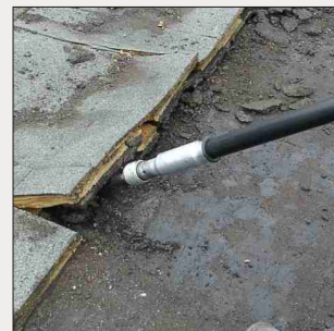
Cut open and remove roof insulation
